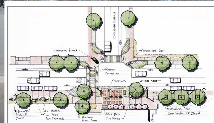
COOLIDGE AVENUE KIMBALL ELEMENTARY SCHOOL CONCEPT PLAN SAFE ROUTES TO SCHOOL NATIONAL CITY, CALIFORNIA
