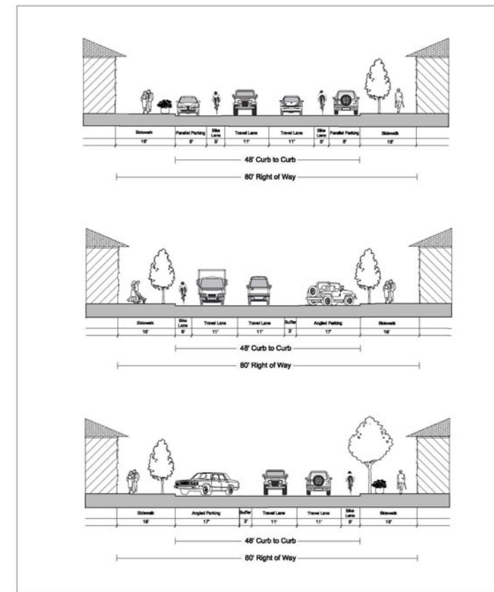
fp FEHR & PEERS TRANSPORTATION CONSULTANTS Jan 29, 2010 5P N:\Jobs\active\OC Jobs\0029-0145\ACAD\0029-0145-Cross Sections.dwg NATIONAL CITY PROPOSED COMMUNITY CORRIDORS STREET CROSS-SECTIONS FIGURE 3
