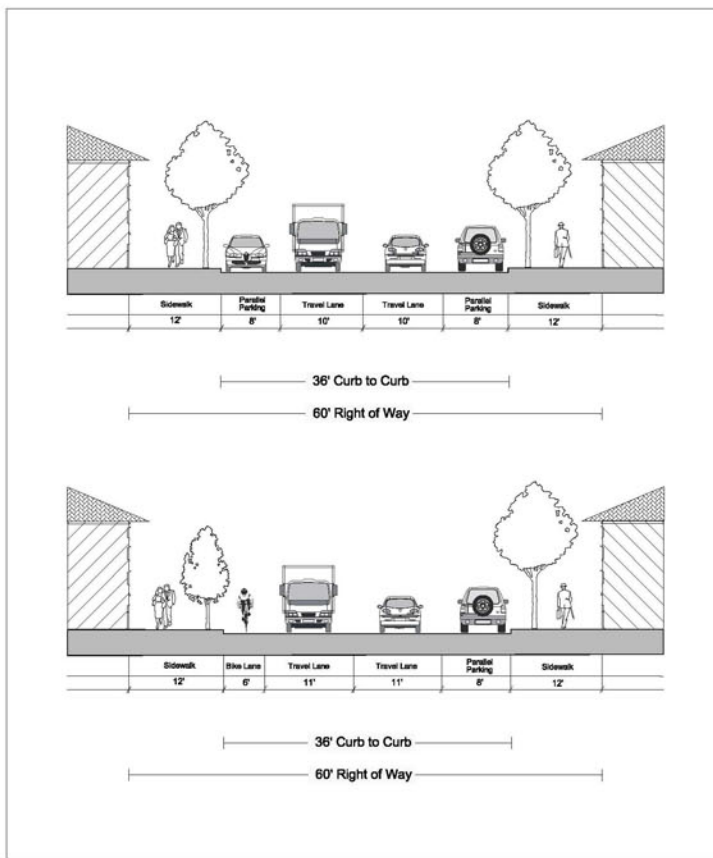
fp FEHR & PEERS TRANSPORTATION CONSULTANTS Jan 29, 2010 5P N:\Jobs\active\OC Jobs\0029-0145\ACAD\0029-0145-Cross Sections.dwg NATIONAL CITY PROPOSED COMMUNITY CORRIDORS STREET CROSS-SECTIONS FIGURE 1
