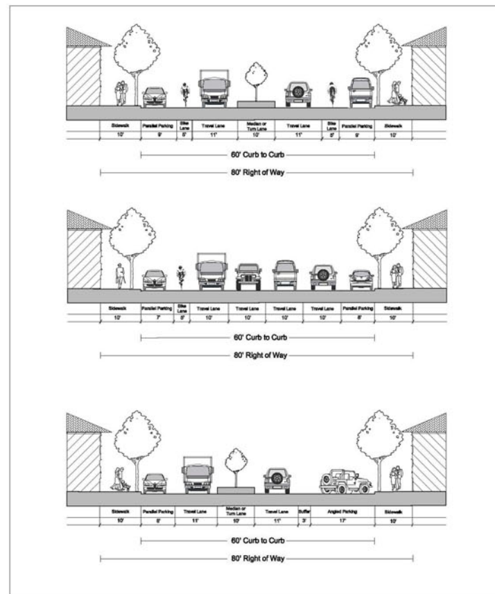
fp FEHR & PEERS TRANSPORTATION CONSULTANTS Jan 29, 2010 5P N:\Jobs\active\OC Jobs\0029-0145\ACAD\0029-0145-Cross Sections.dwg NATIONAL CITY PROPOSED COMMUNITY CORRIDORS STREET CROSS-SECTIONS FIGURE 5
