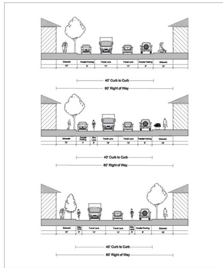
fp FEHR & PEERS TRANSPORTATION CONSULTANTS Jan 29, 2010 5P N:\Jobs\active\OC Jobs\0029-0145\ACAD\0029-0145-Cross Sections.dwg NATIONAL CITY PROPOSED COMMUNITY CORRIDORS STREET CROSS-SECTIONS FIGURE 2
