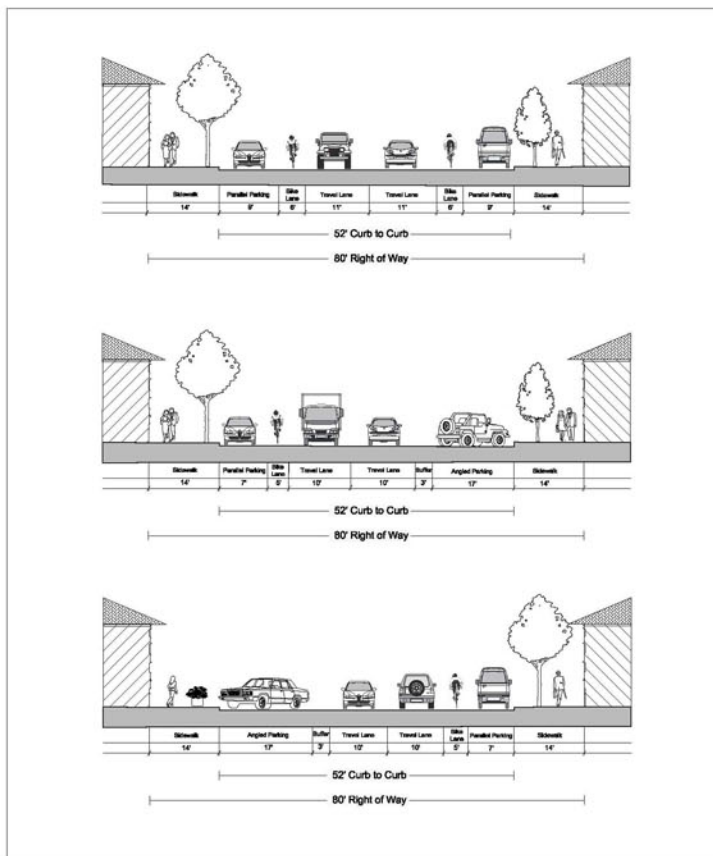
fp FEHR & PEERS TRANSPORTATION CONSULTANTS Jan 29, 2010 5P N:\Jobs\active\OC Jobs\0029-0145\ACAD\0029-0145-Cross Sections.dwg NATIONAL CITY PROPOSED COMMUNITY CORRIDORS STREET CROSS-SECTIONS FIGURE 4
